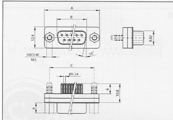
Socket connector
