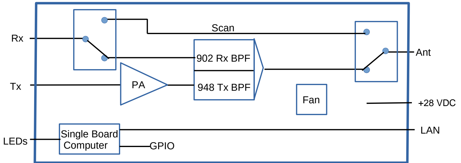
Module Block Diagram
